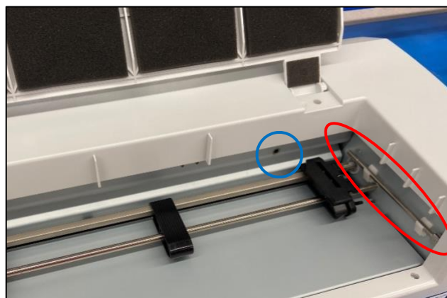
Shows the shipping bolt removed (blue) and how to store (red)
